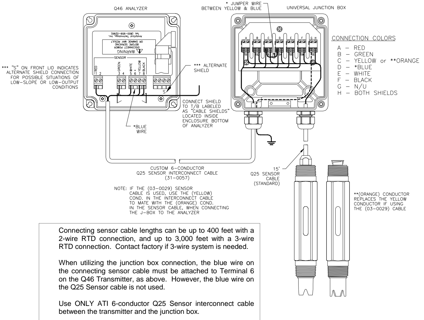
Figure 25 - Junction Box Interconnect Wiring
