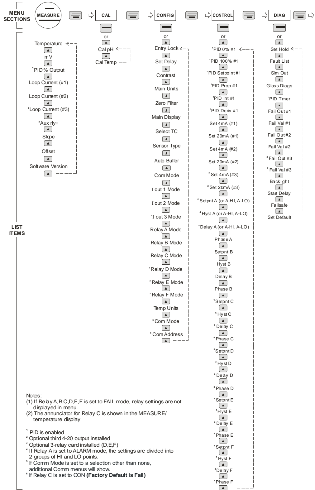
Figure 30 - Software Map
